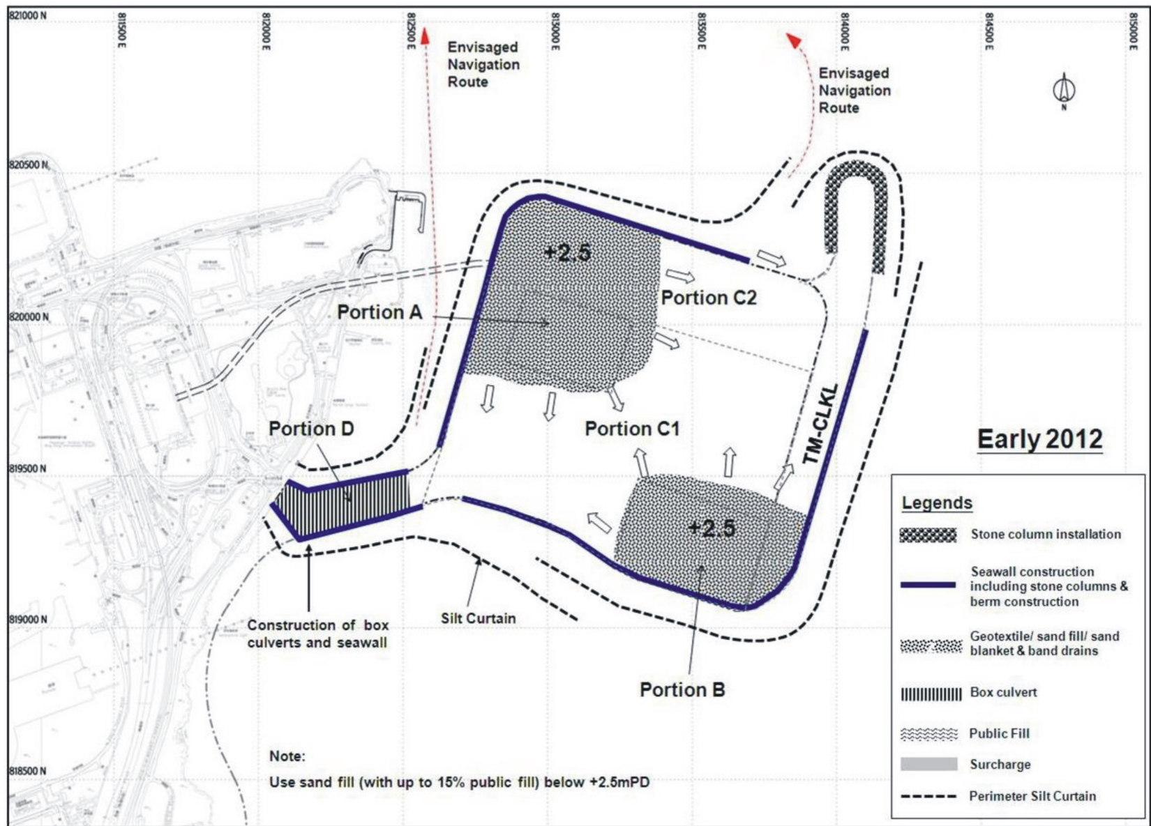
Figure 14 - Outline of Construction Sequence (Sheet 3 of 10)
